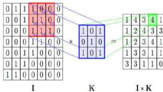
Fig 2. Convolutional layer
