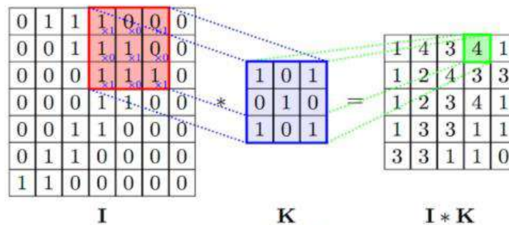
Fig 2. Convolutional layer
